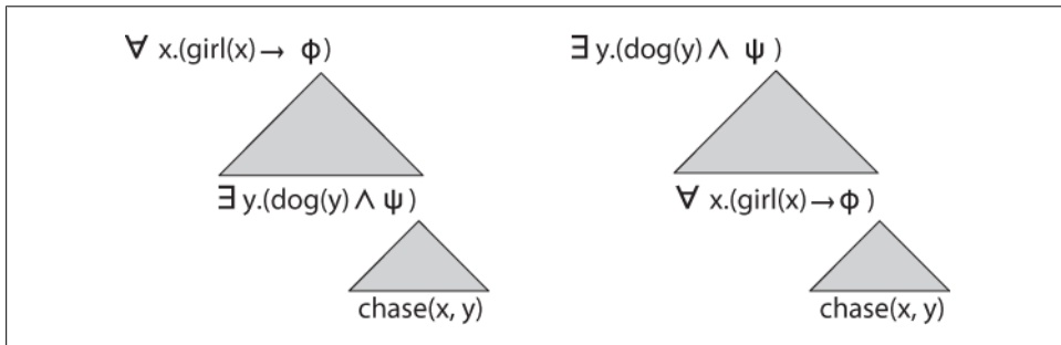
Figure 10-3. Quantifier scopings.
